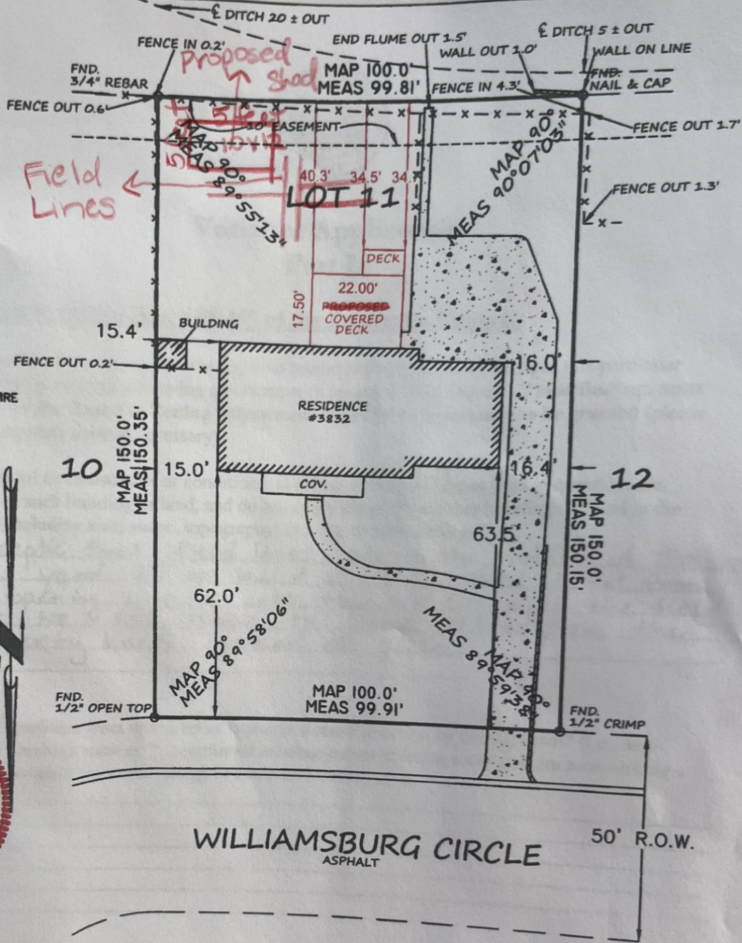
"Plot Plan"
