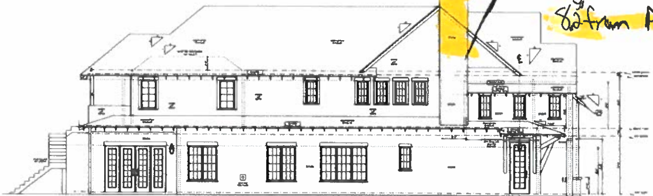
LEFT ELEVATION DETAIL SCALE 1/8" = 1'-0"
