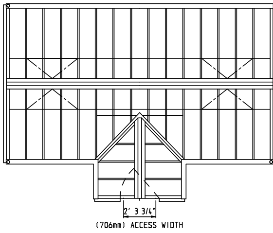
AERIAL PLAN
