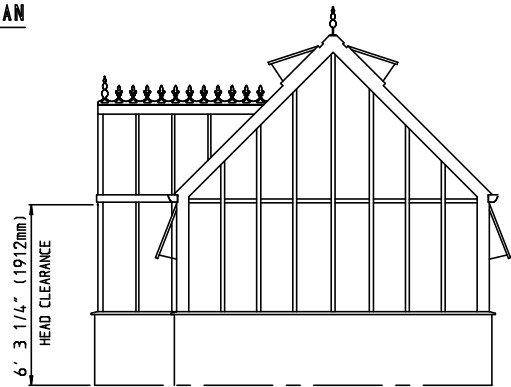
RIGHT ELEVATION PLAN
