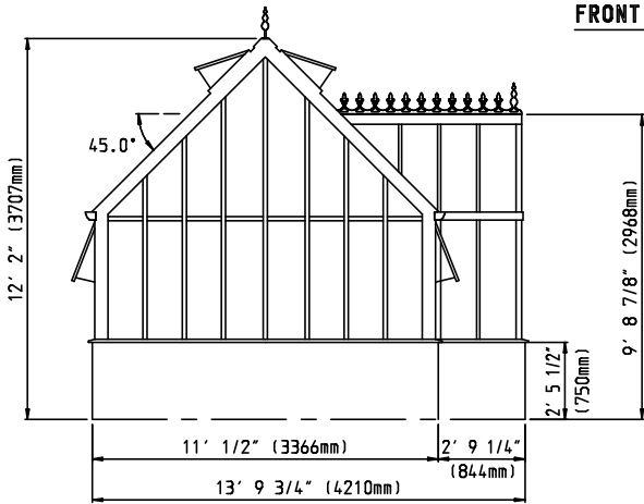
LEFT ELEVATION PLAN
