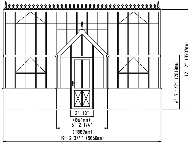
FRONT ELEVATION PLAN
