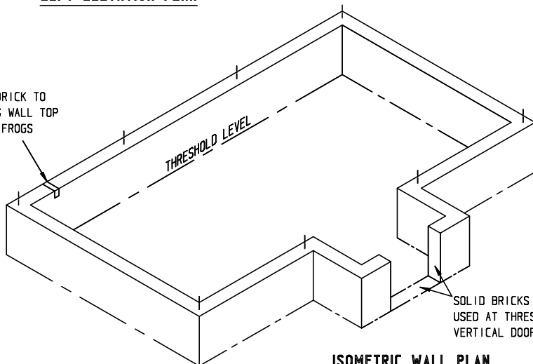
ISOMETRIC WALL PLAN
