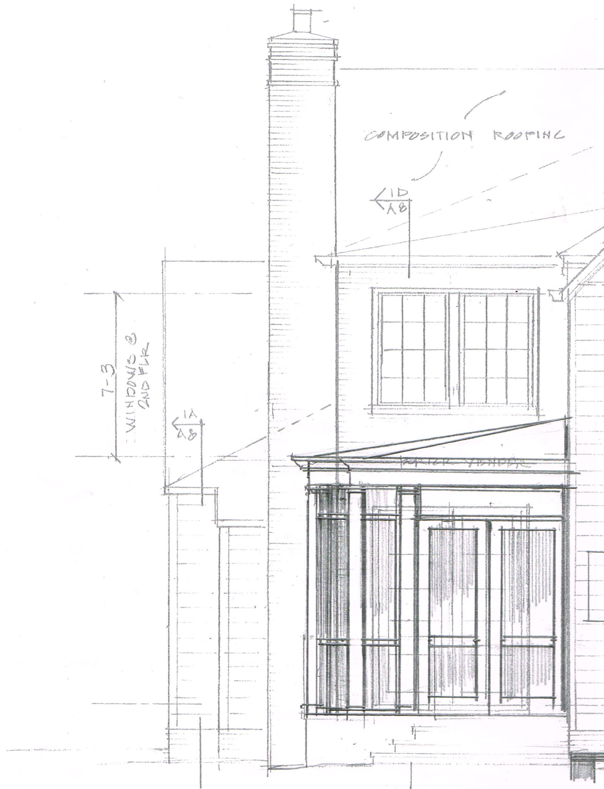
REAR ELEV @ SCREENED TERRACE
