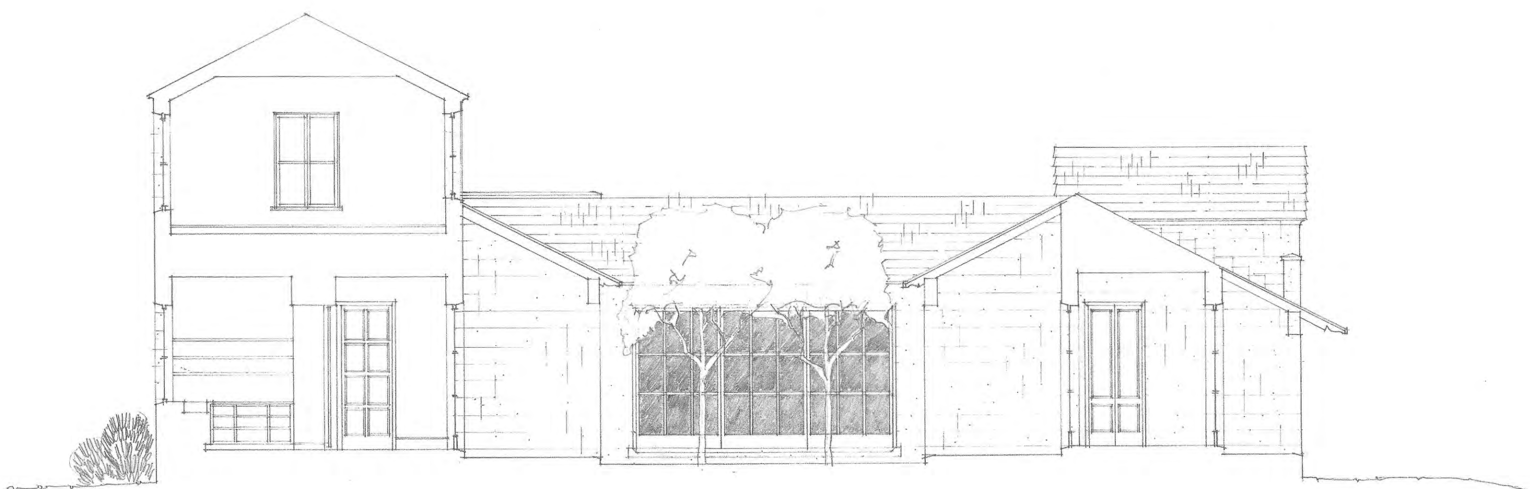
courtyard section toward master
