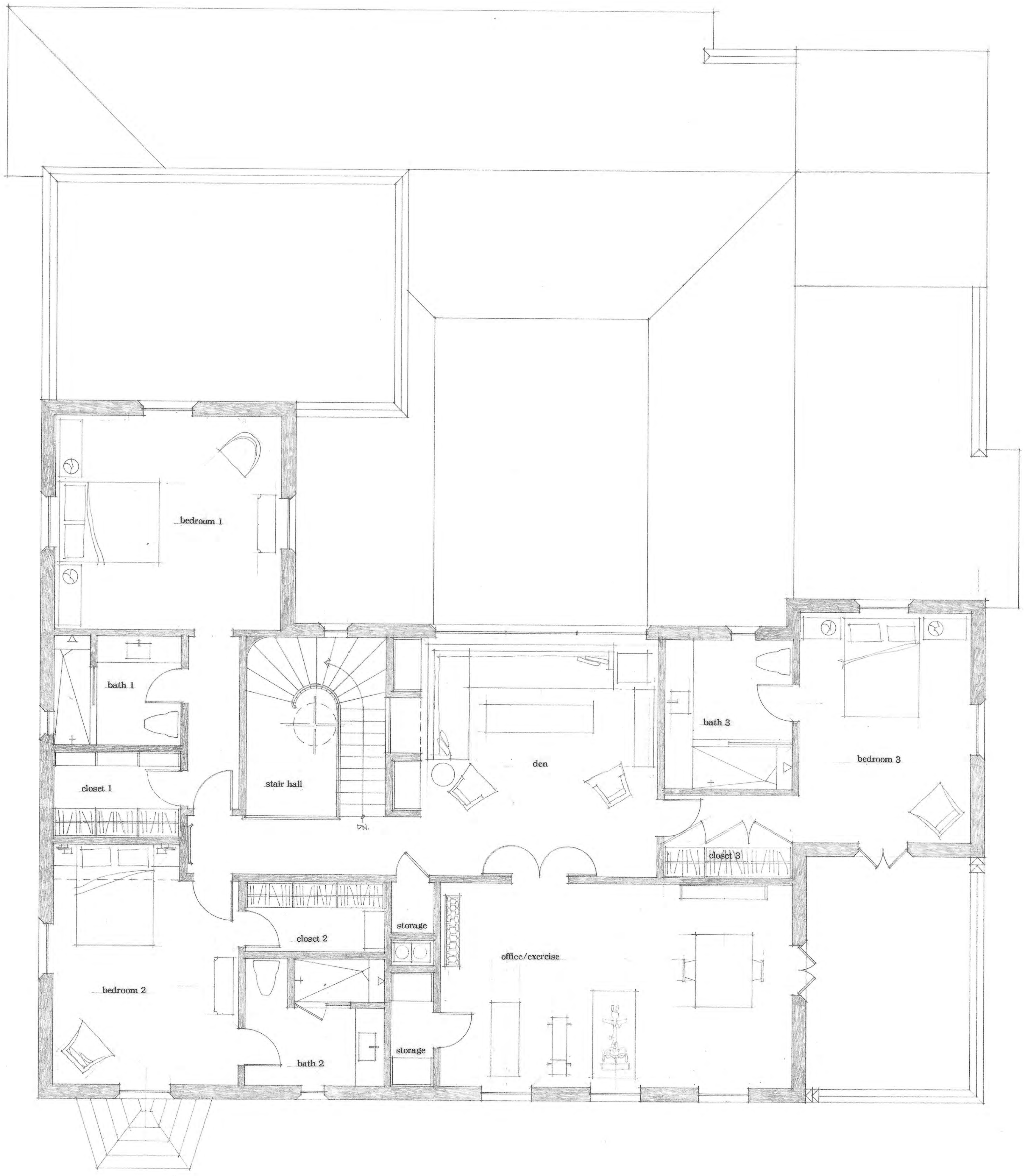
second floor plan 1/4" = 1'-0"
