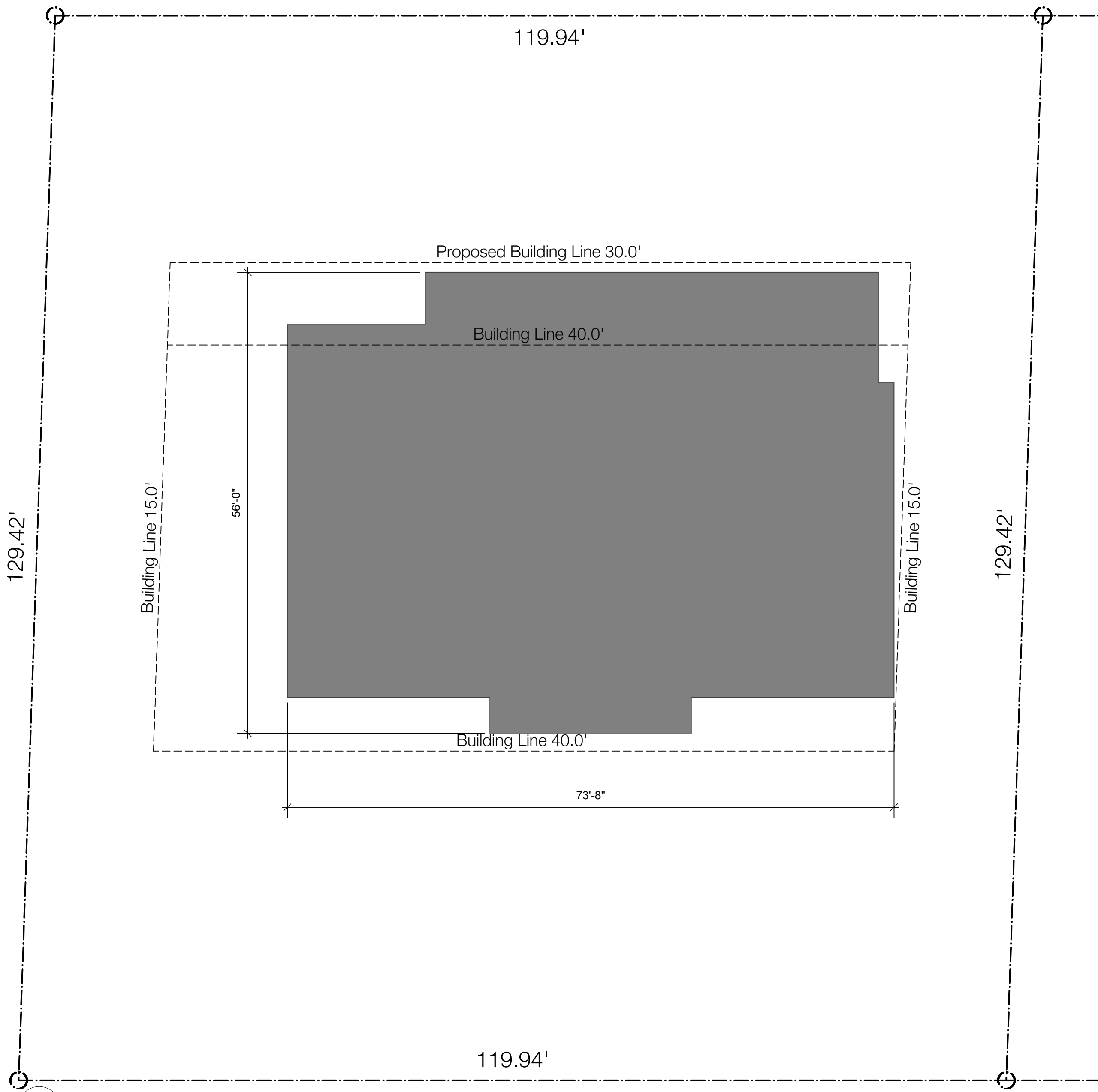
1 Architectural Site Plan A0.1 Scale: 1" = 10 ft
