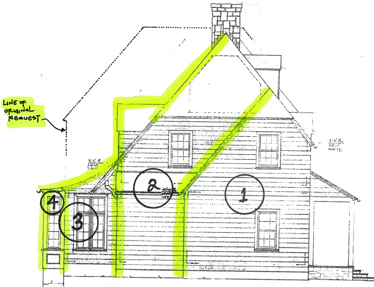
LEFT SIDE ELEVATION (south)
